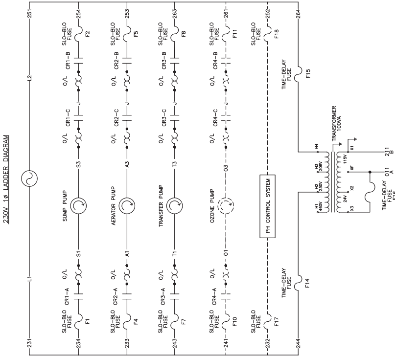
LADDER DIAGRAM - MASTER - BIO-20R, 25R, 35R - 1 PHASE 091616
